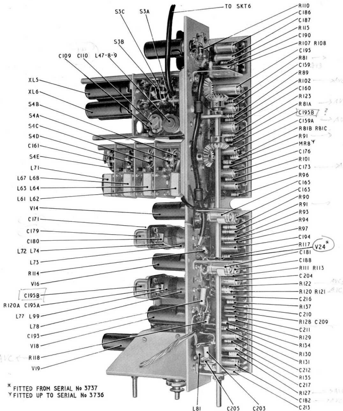
100 KC/S I.F. STRIP (RIGHT SIDE)
