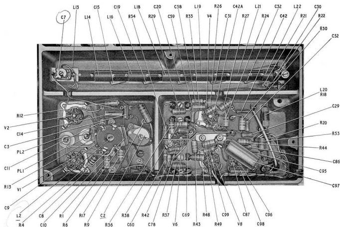
CRYSTAL OSCILLATOR AND HARMONIC FILTER SYSTEM (UNDERSIDE)
