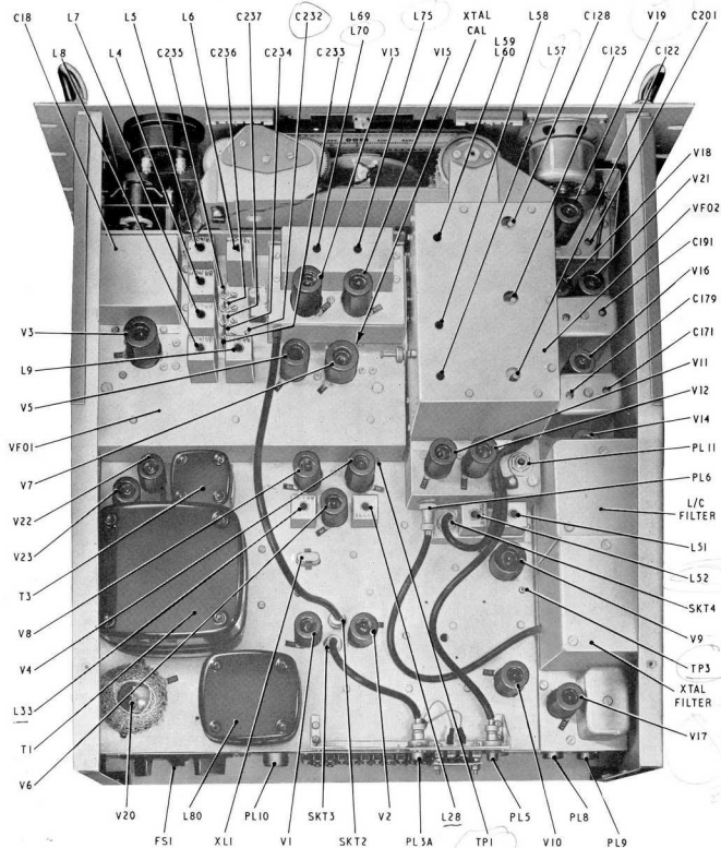
CHASSIS ASSEMBLY (TOP)
