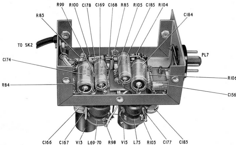
CRYSTAL CALIBRATOR UNIT (UNDERSIDE)
