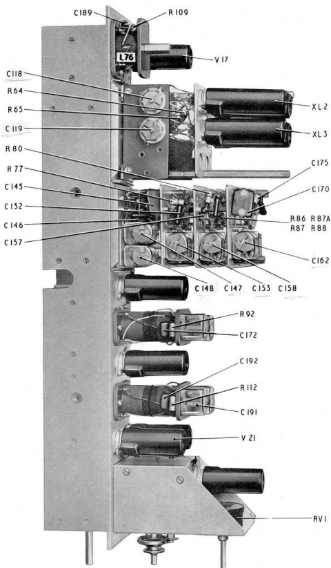
100 KC/S I.F. STRIP (LEFT SIDE)
