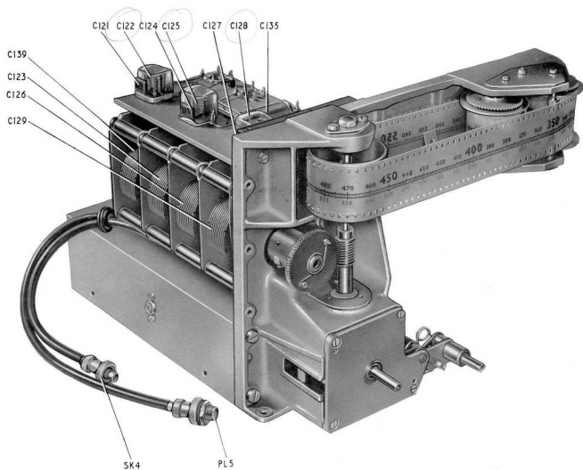
SECOND VFO UNIT (FRONT)
